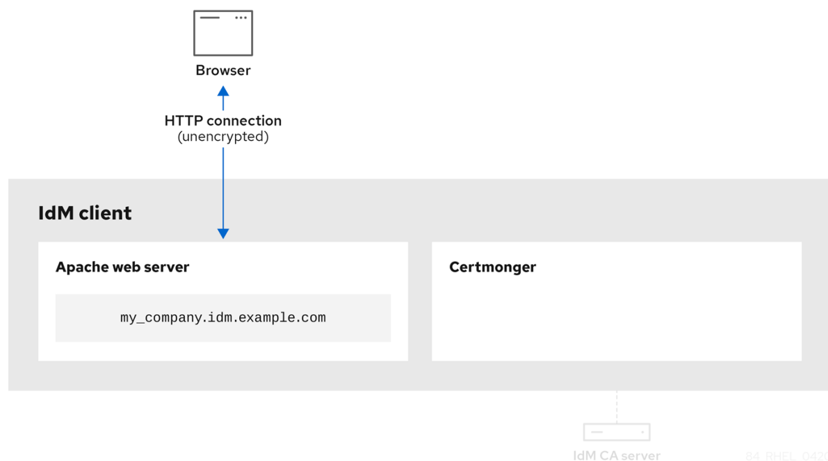
Figure 17.3. Unencrypted communication
