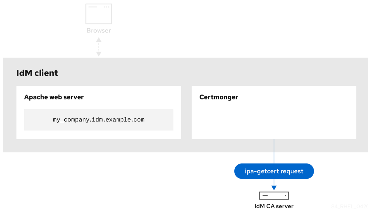
Figure 17.4. Certmonger requesting a service certificate
