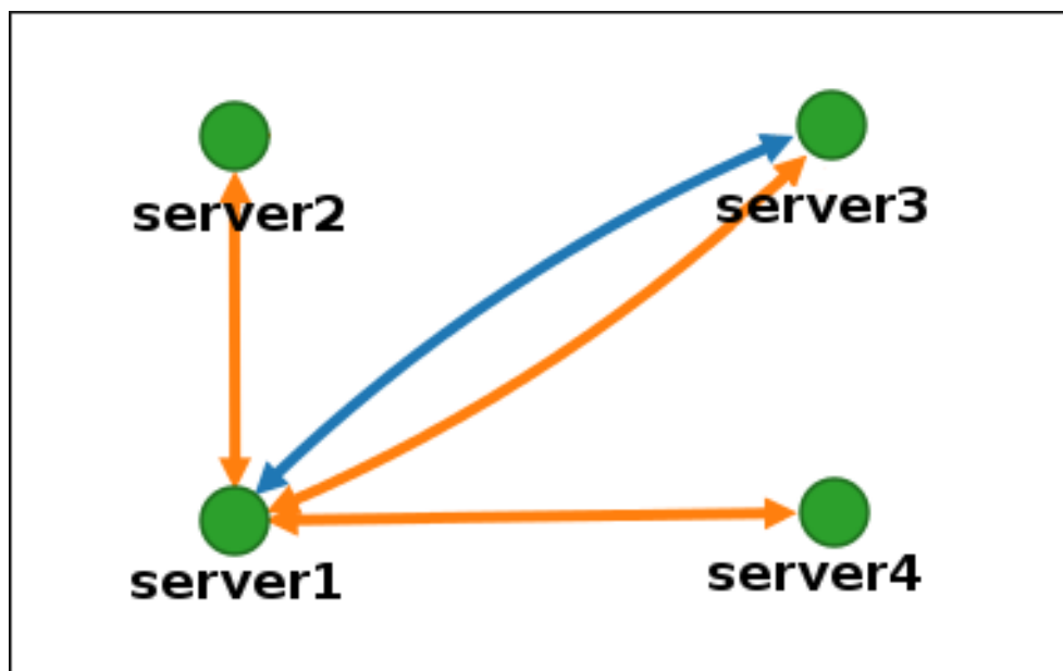
Figure 54.5. Discouraged topology example: Single Point of Failure
