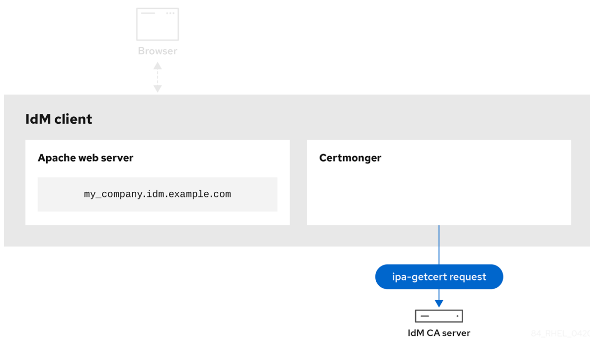
Figure 70.2. Certmonger requesting a service certificate
