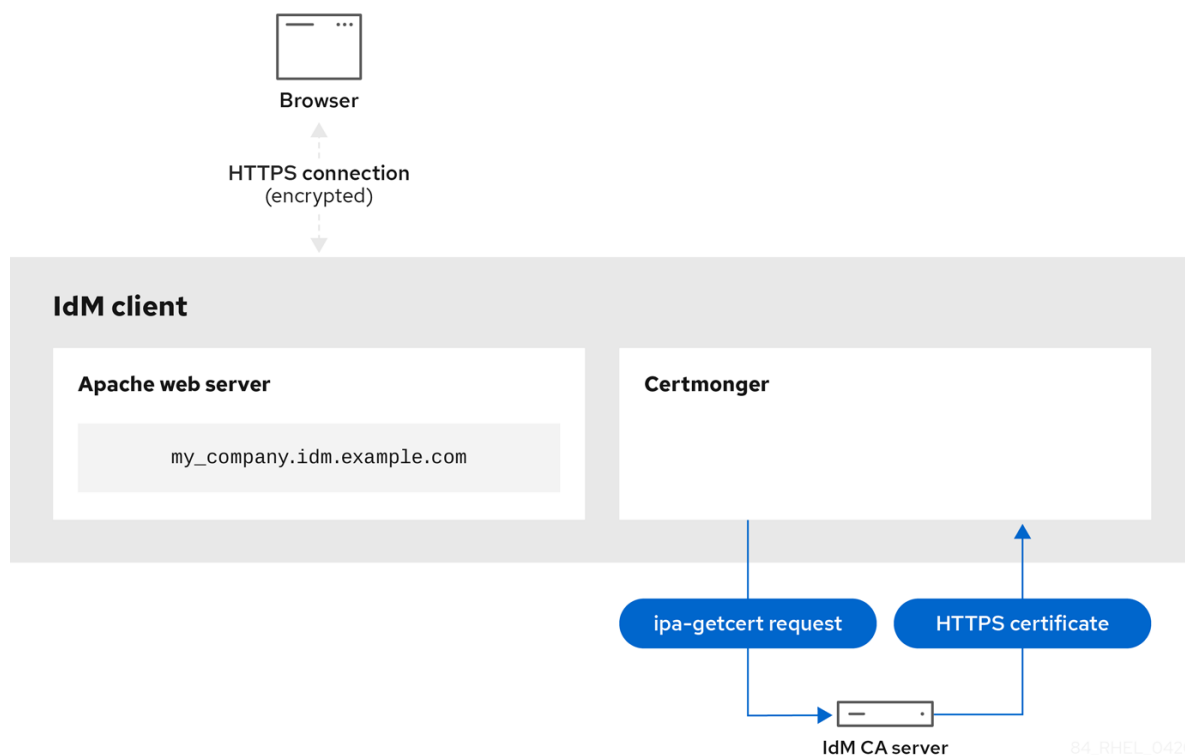
Figure 70.5. Certmonger requesting a new certificate when the old one is nearing expiration
