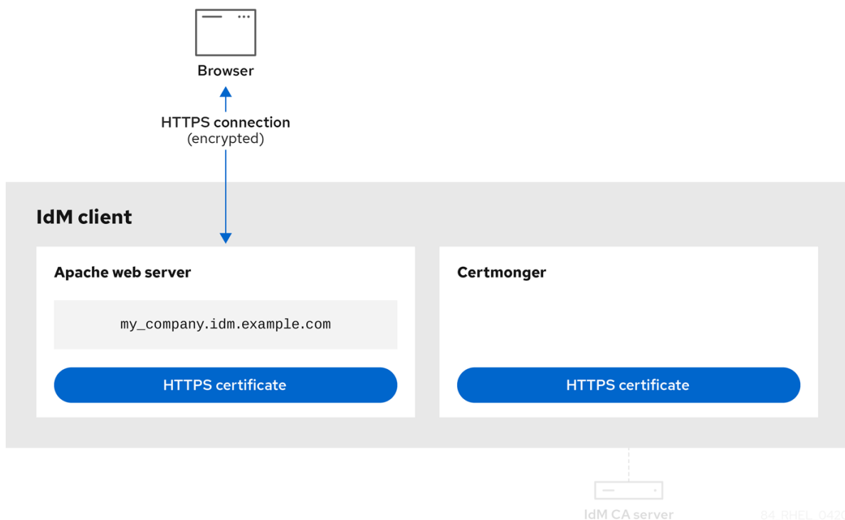
Figure 72.6. Certmonger applying the service certificate
