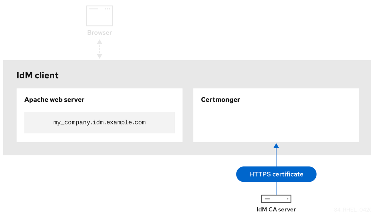
Figure 70.3. IdM CA issuing the service certificate
