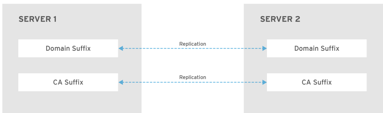
Figure 54.2. Topology suffixes
