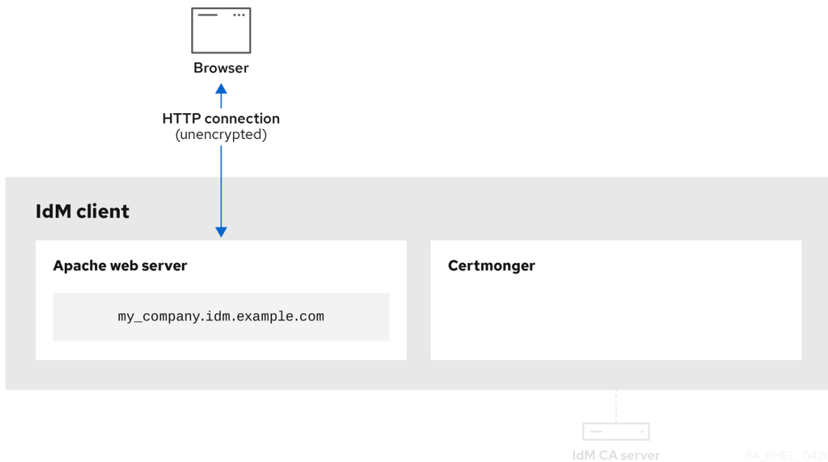
Figure 70.1. Unencrypted communication
