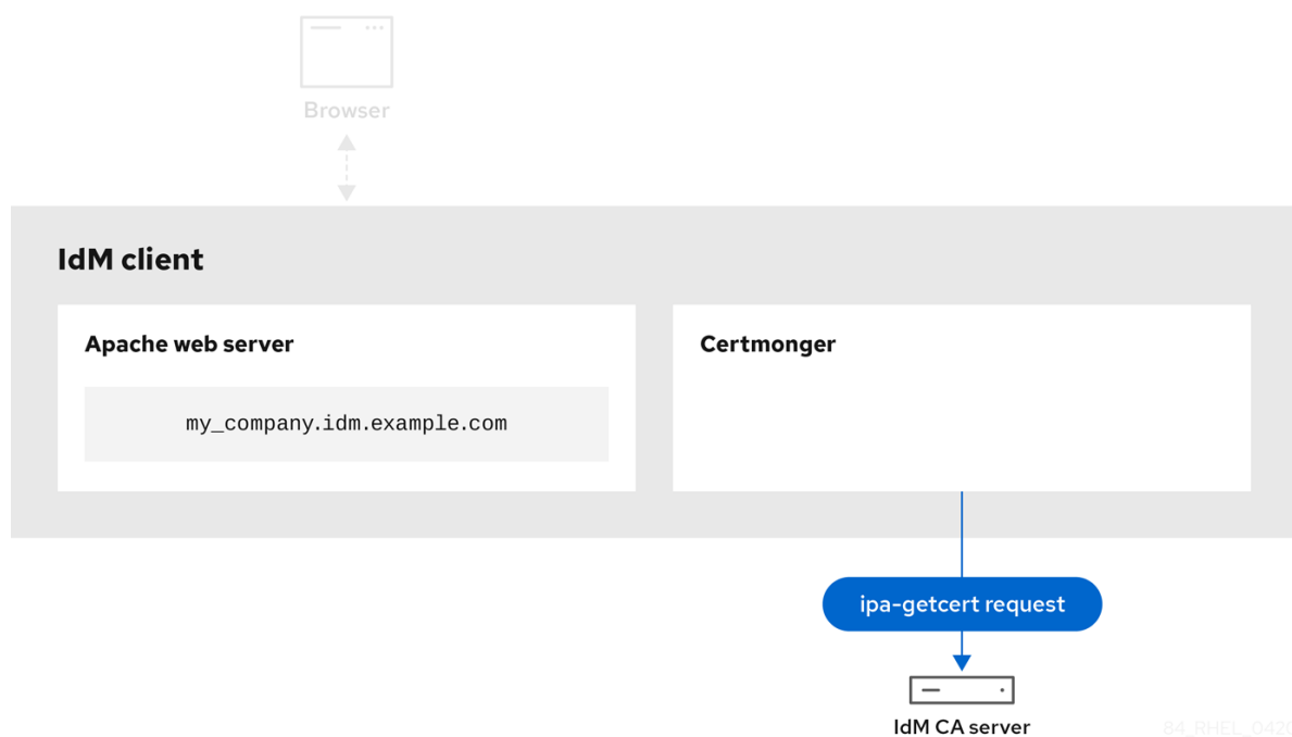
Figure 72.4. Certmonger requesting a service certificate
