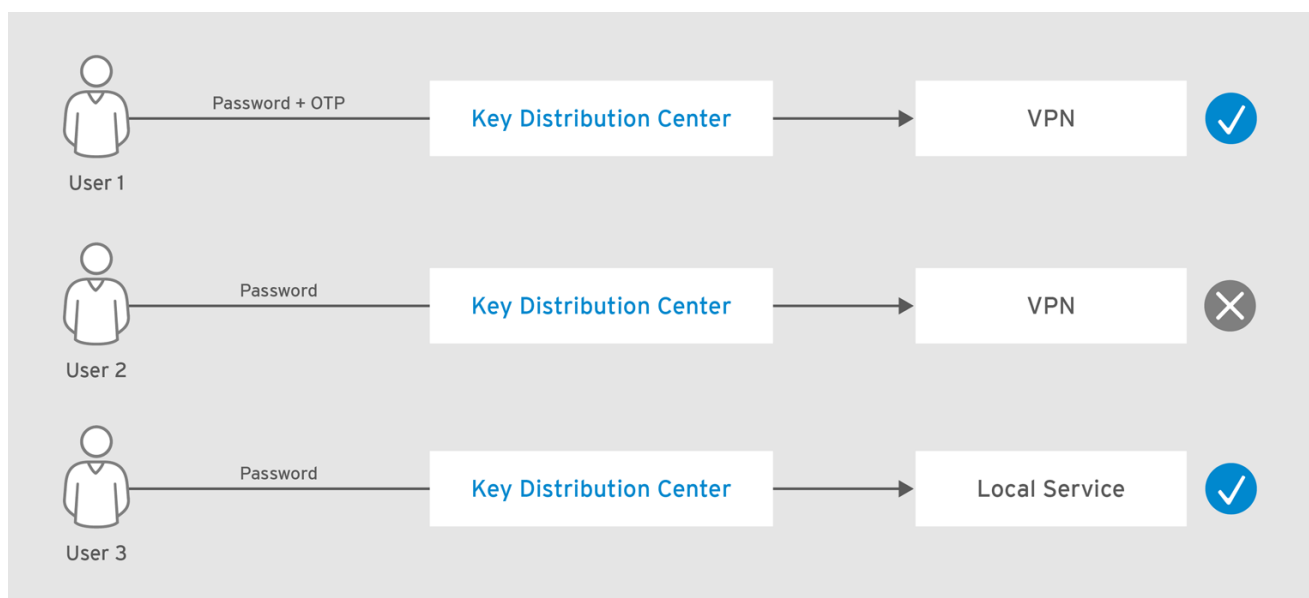
Figure 47.1. Example of authenticating using different technologies
