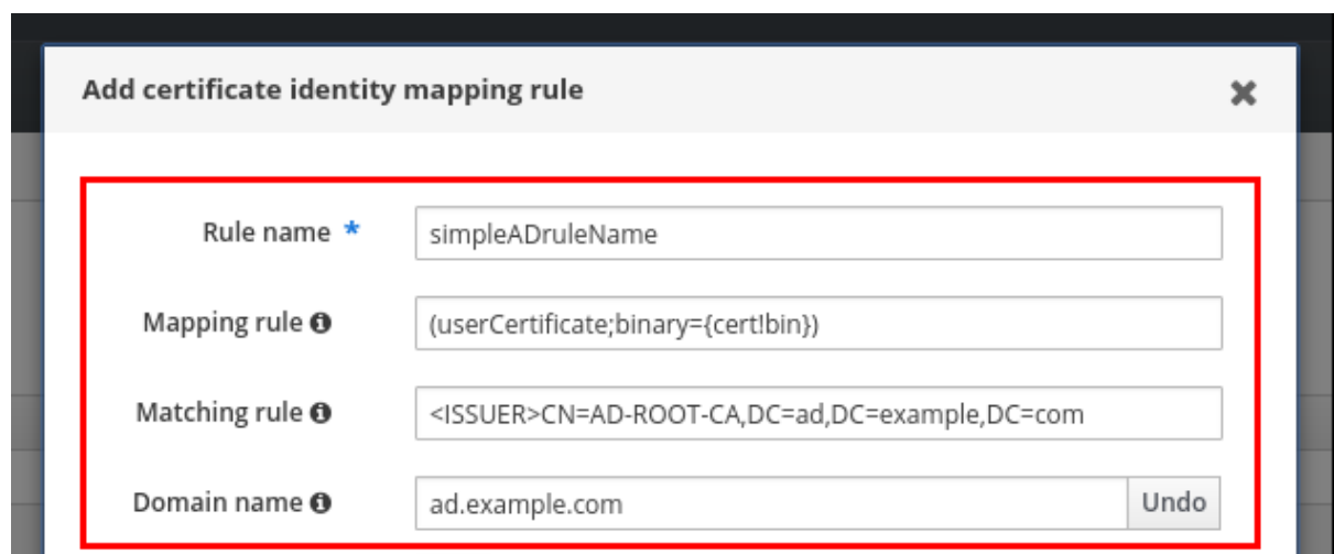
Figure 63.10. Certificate mapping rule for a user with no certificate or mapping data stored in AD
