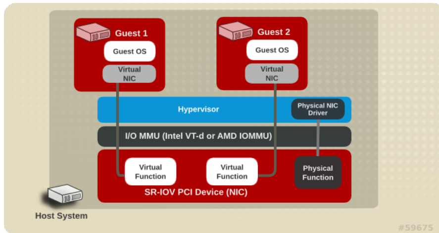
Figure 13.1. How SR-IOV works
