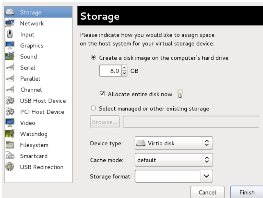
Figure 10.24. The virtual machine hardware information window
