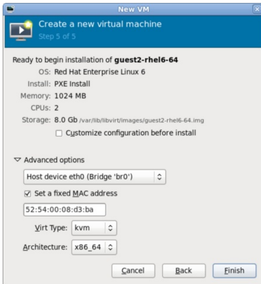
Figure 7.18. The New VM window - Step 5 - PXE Install
