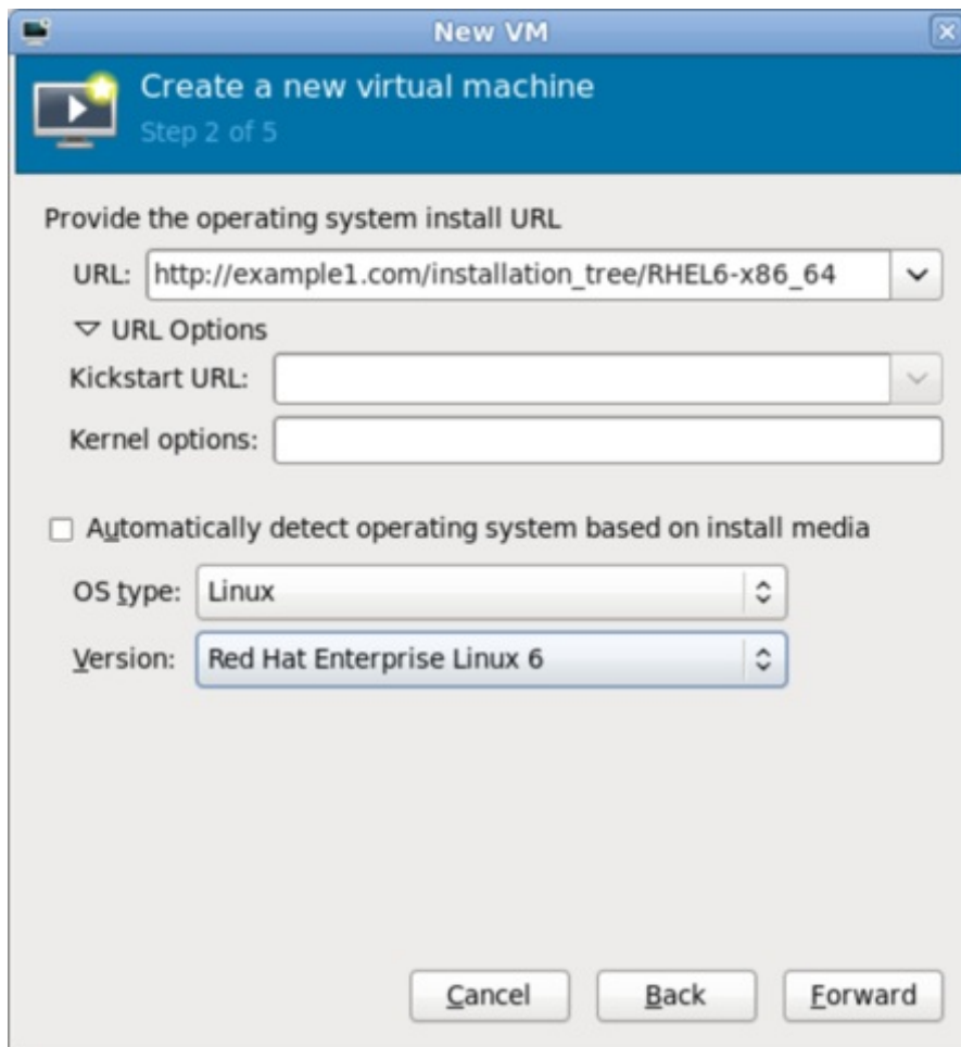
Figure 7.14. The New VM window - Step 2
