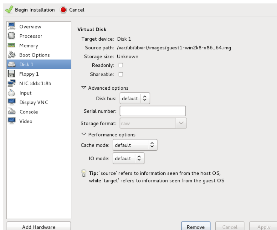
Figure 10.23. The virtual machine hardware information window
