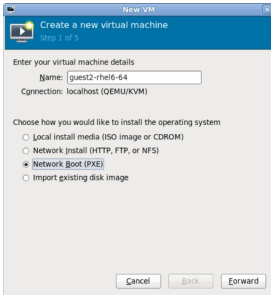
Figure 6.8. Selecting the installation method
