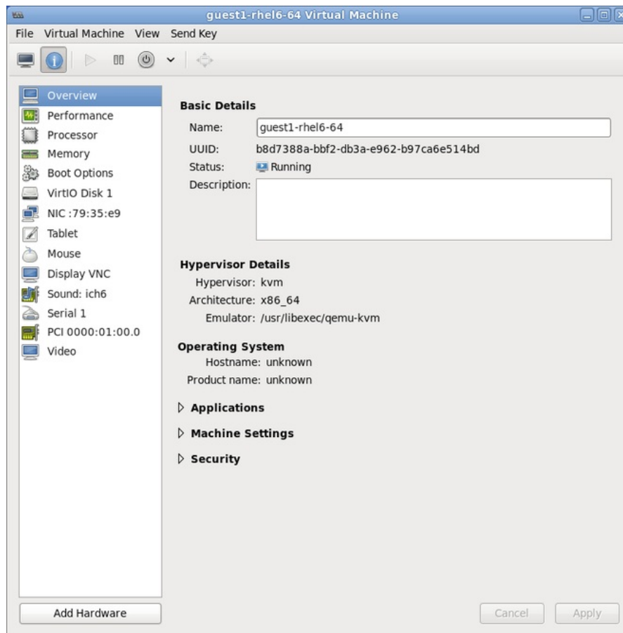
Figure 12.3. The virtual machine hardware information window
