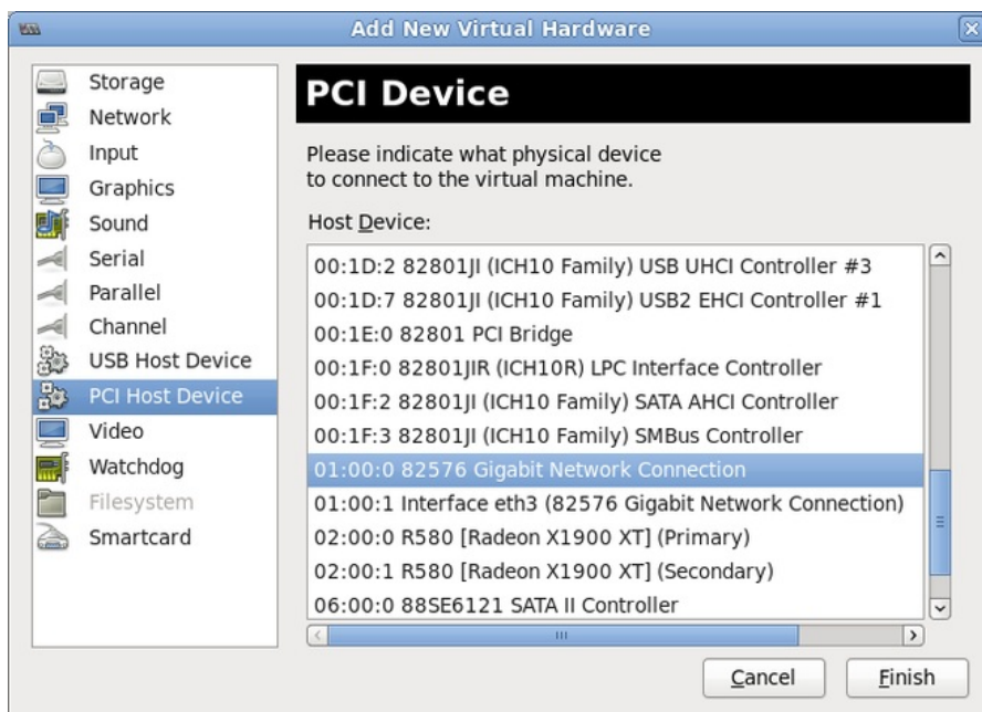
Figure 12.2. The Add new virtual hardware wizard
