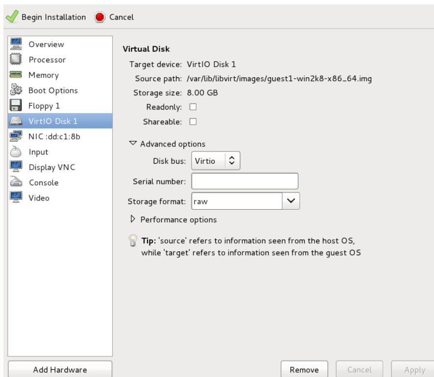
Figure 10.25. The virtual machine hardware information window
