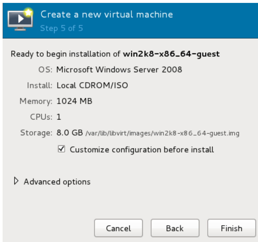
Figure 10.17. The virt-manager guest creation wizard
