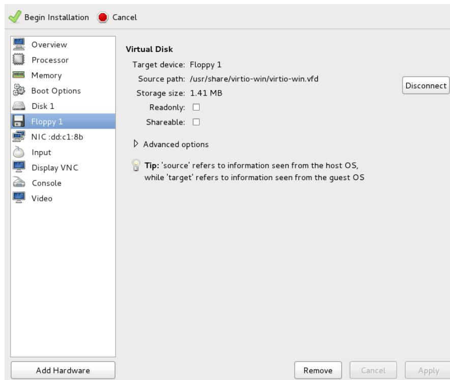
Figure 10.22. The virtual machine hardware information window
