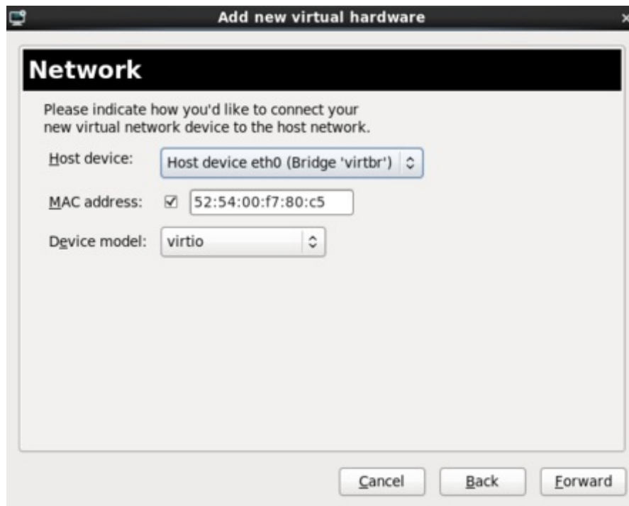
Figure 10.35. The Add new virtual hardware wizard
