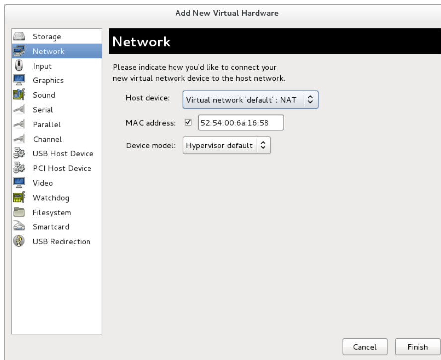
Figure 10.32. The Add new virtual hardware wizard
