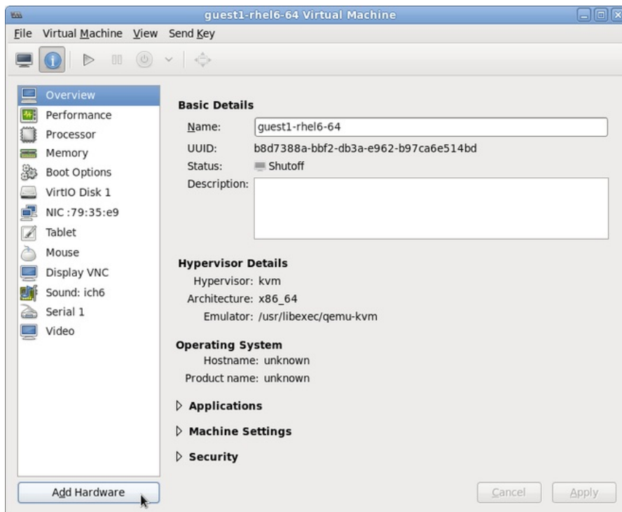
Figure 12.1. The virtual machine hardware information window
