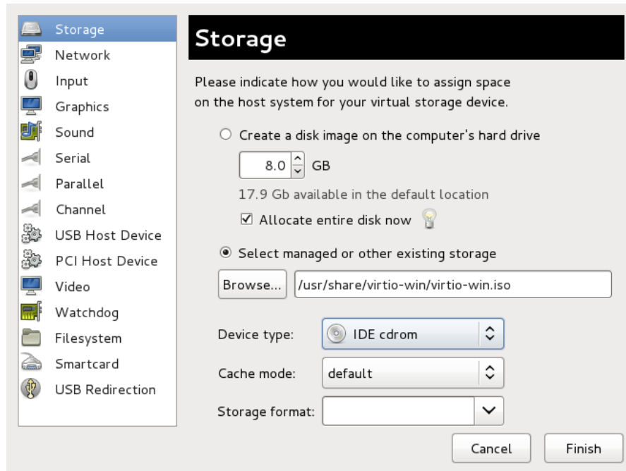
Figure 10.4. The Add new virtual hardware wizard
