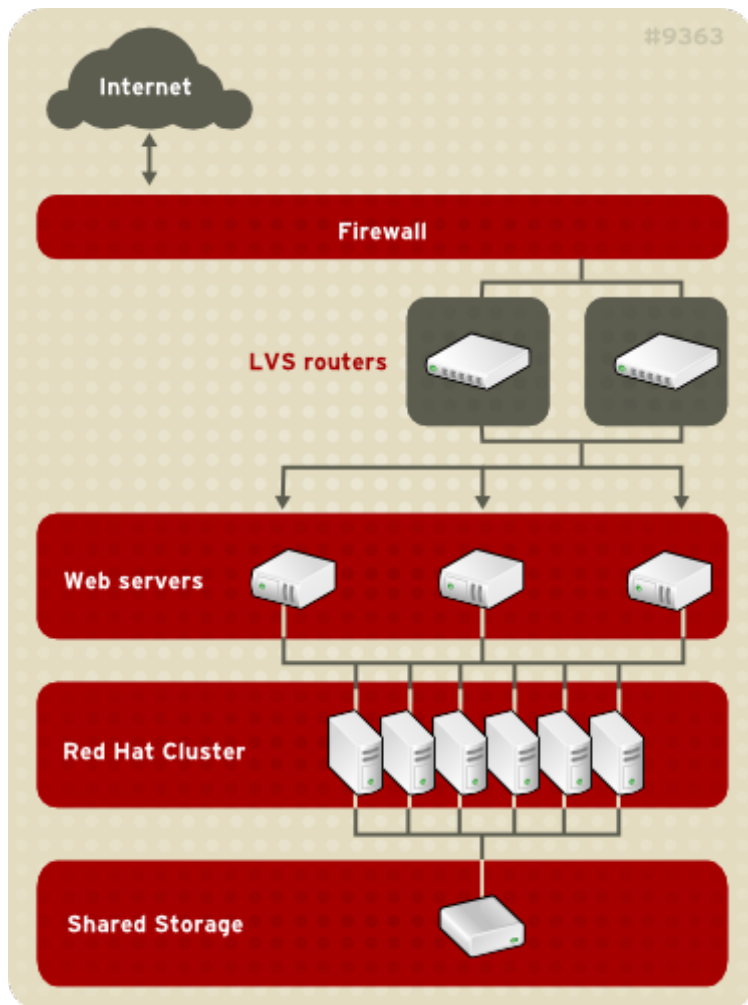
Figure A.1. Load Balancer Add-On with a High Availability Add-On
