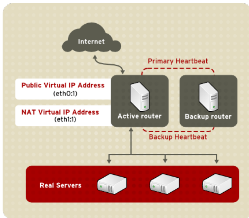
Figure 1.3. Load Balancer Add-On Implemented with NAT Routing
