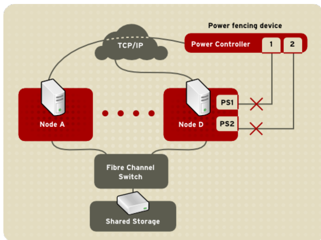
Figure 4.3. Fencing a Node with Dual Power Supplies
