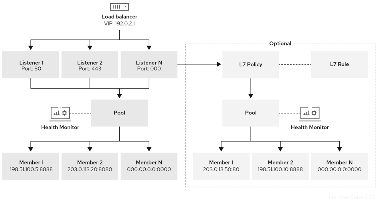
Figure 1.2. Load-balancing service object model diagram
