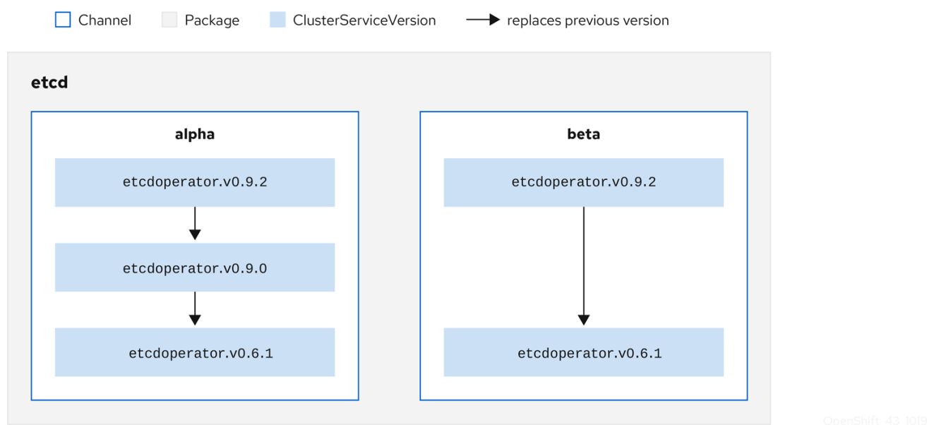
Figure 2.4. Packages and channels in a Catalog source
