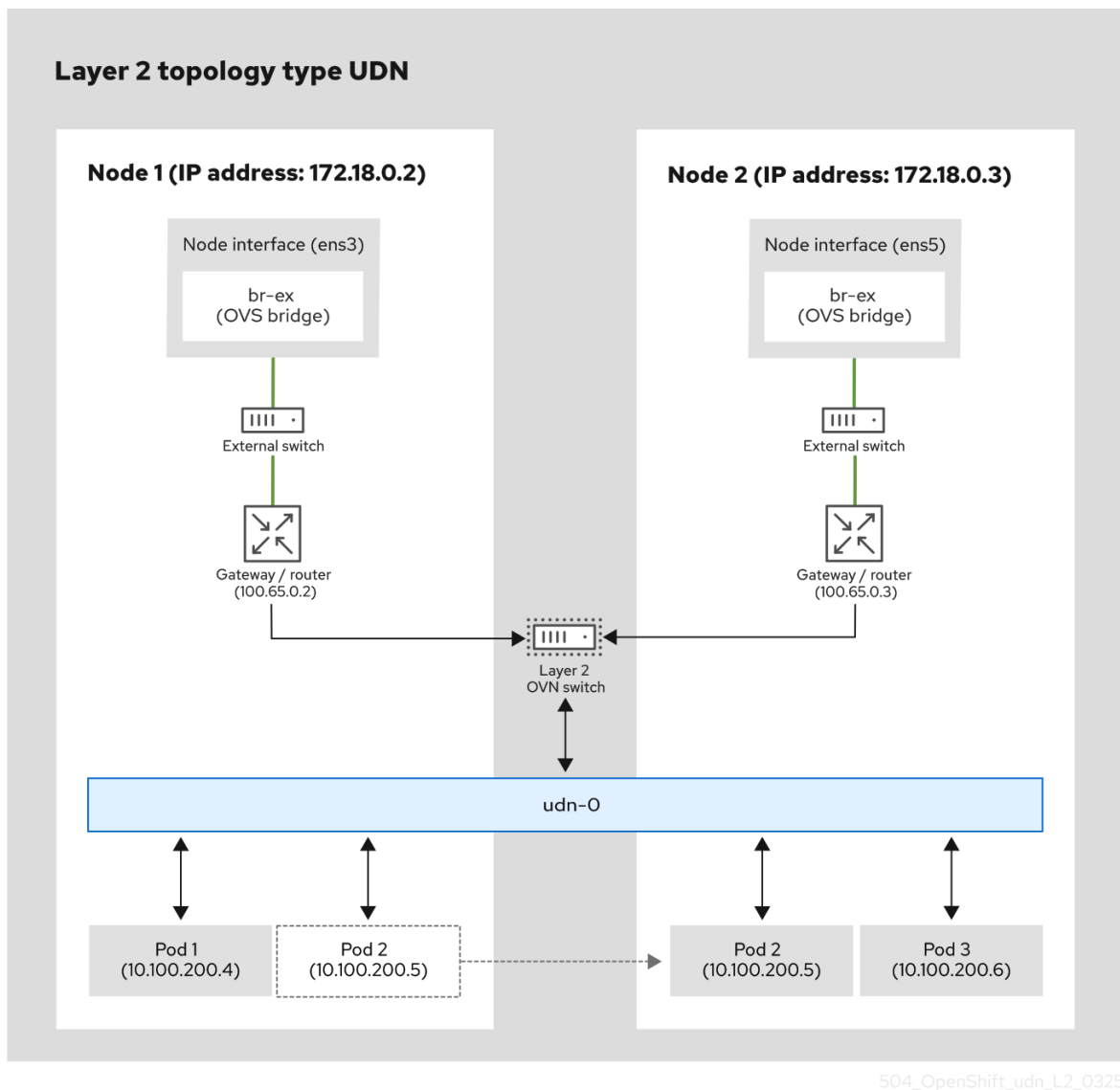
Figure 3.1. A flat layer 2 topology that uses a virtual switch for component communication
