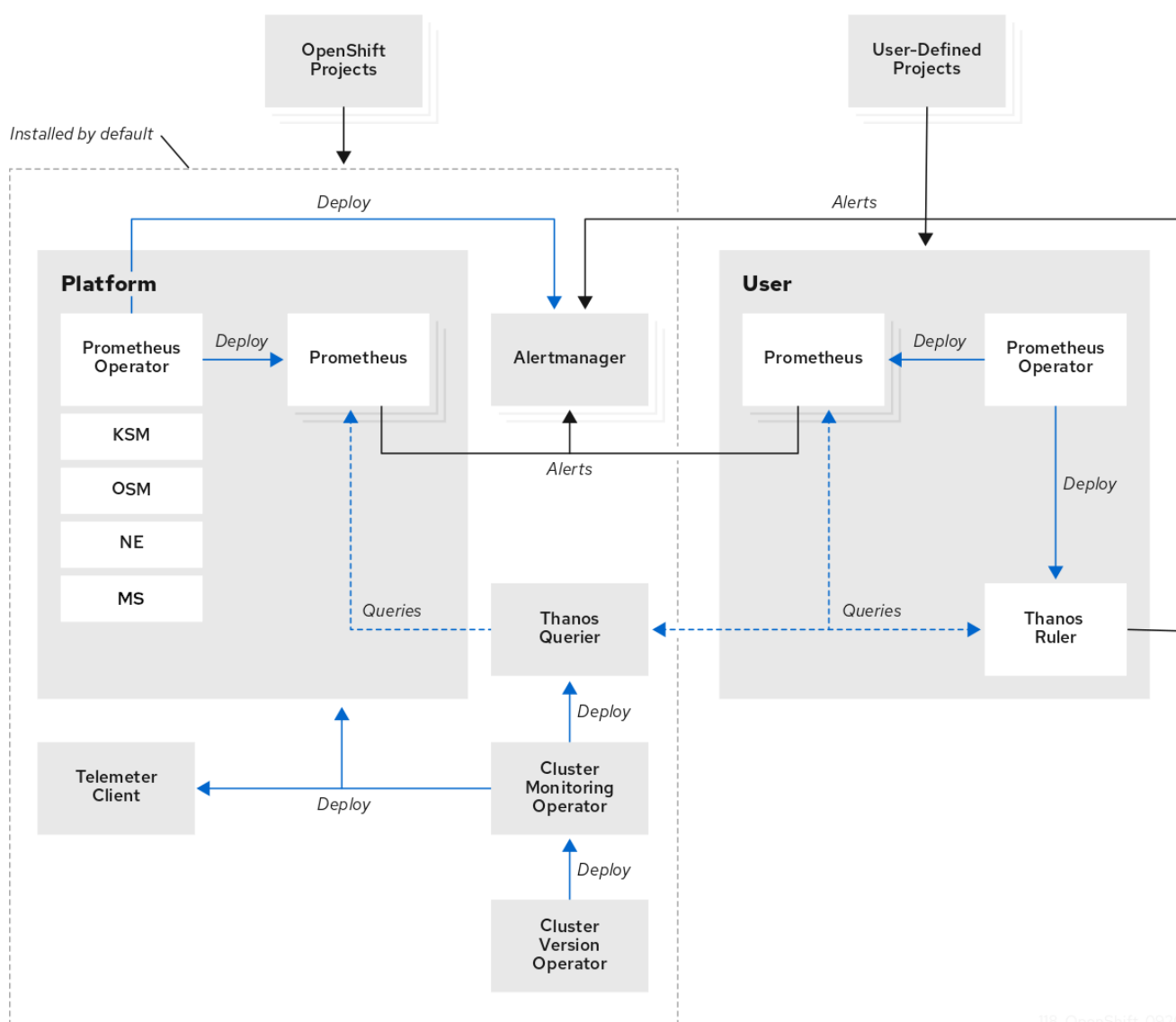
Figure 18.2. OpenShift Container Platform monitoring architecture
