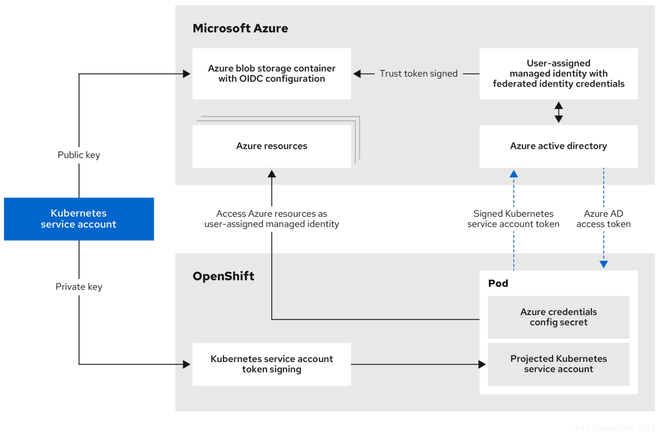
Figure 20.4. Workload ID authentication flow
