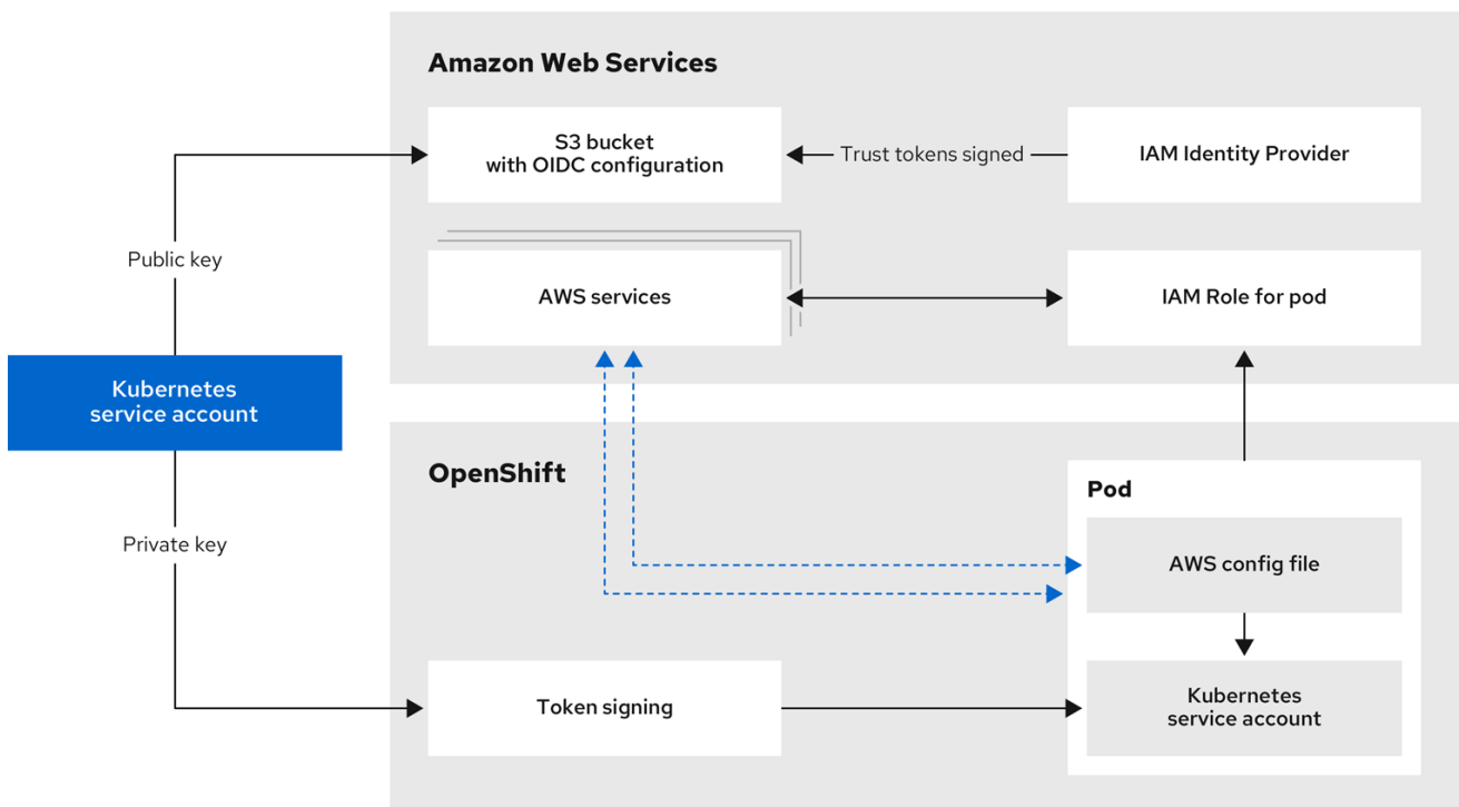
Figure 20.2. AWS Security Token Service authentication flow
