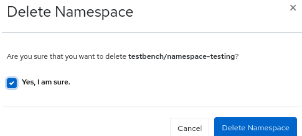
Figure 14.9. Deleting namespaces
