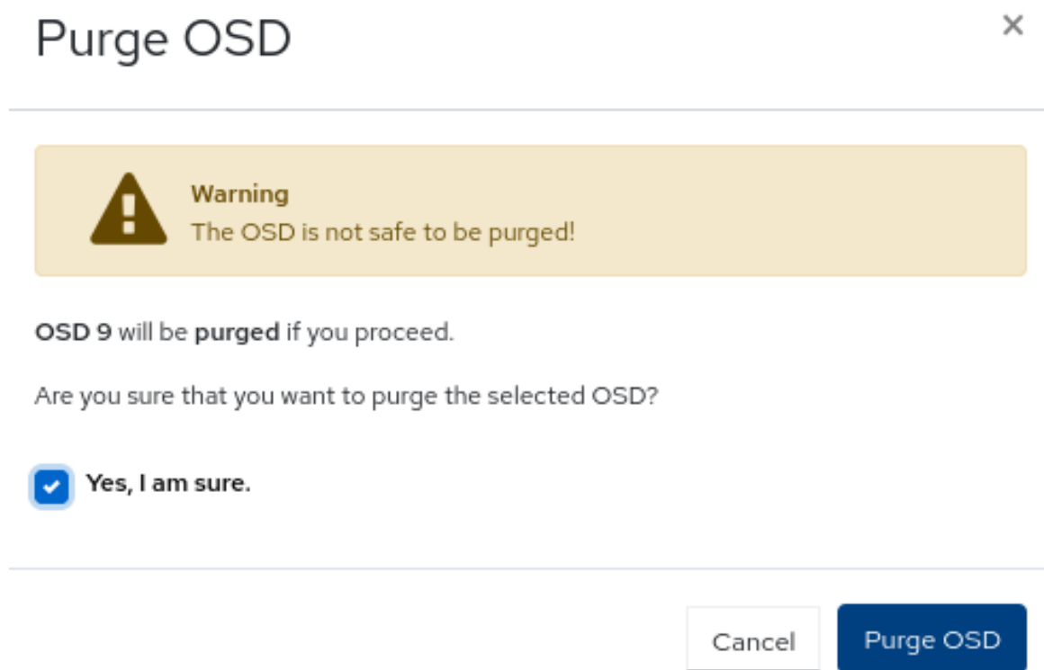
Figure 11.11. Purging OSDs
