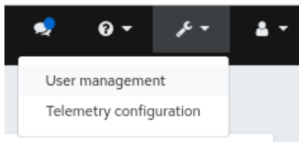
Figure 2.6. User management
