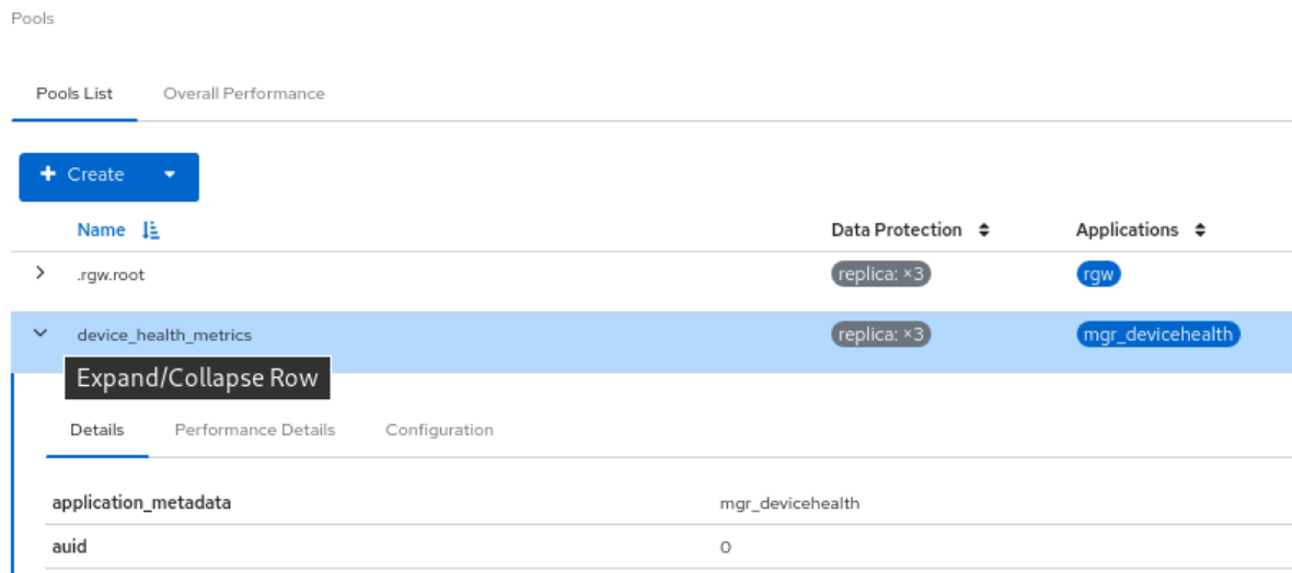
Figure 6.12. Monitoring pools
