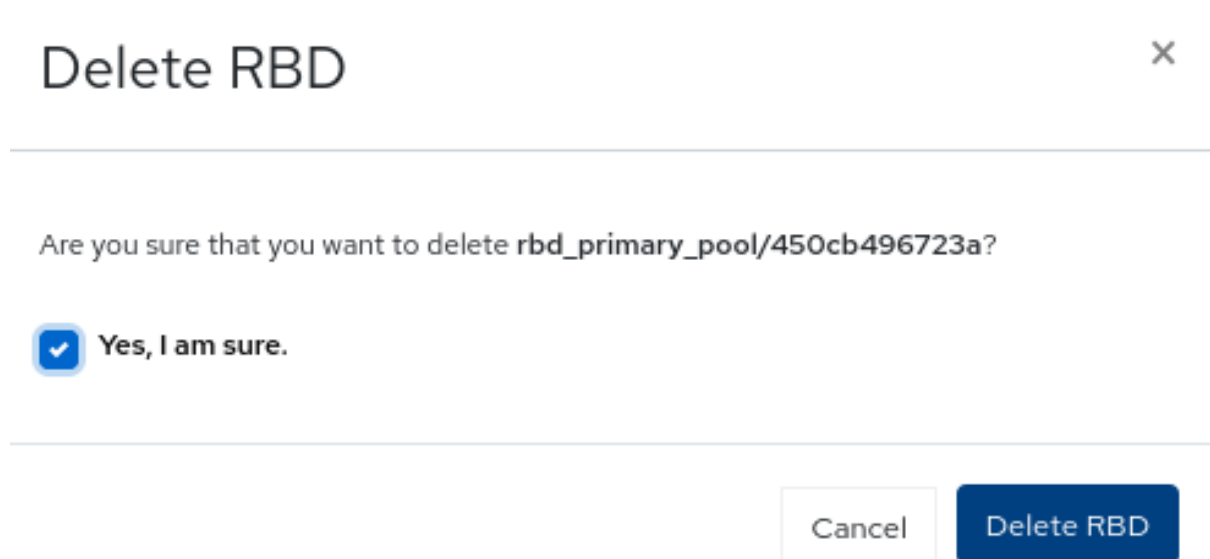
Figure 14.8. Deleting images
