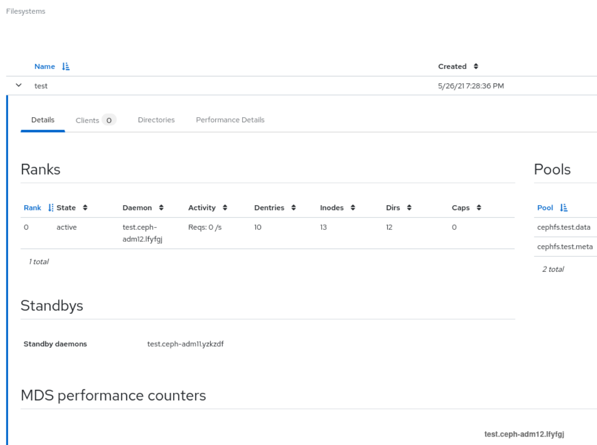
Figure 6.13. Monitoring Ceph File Systems
